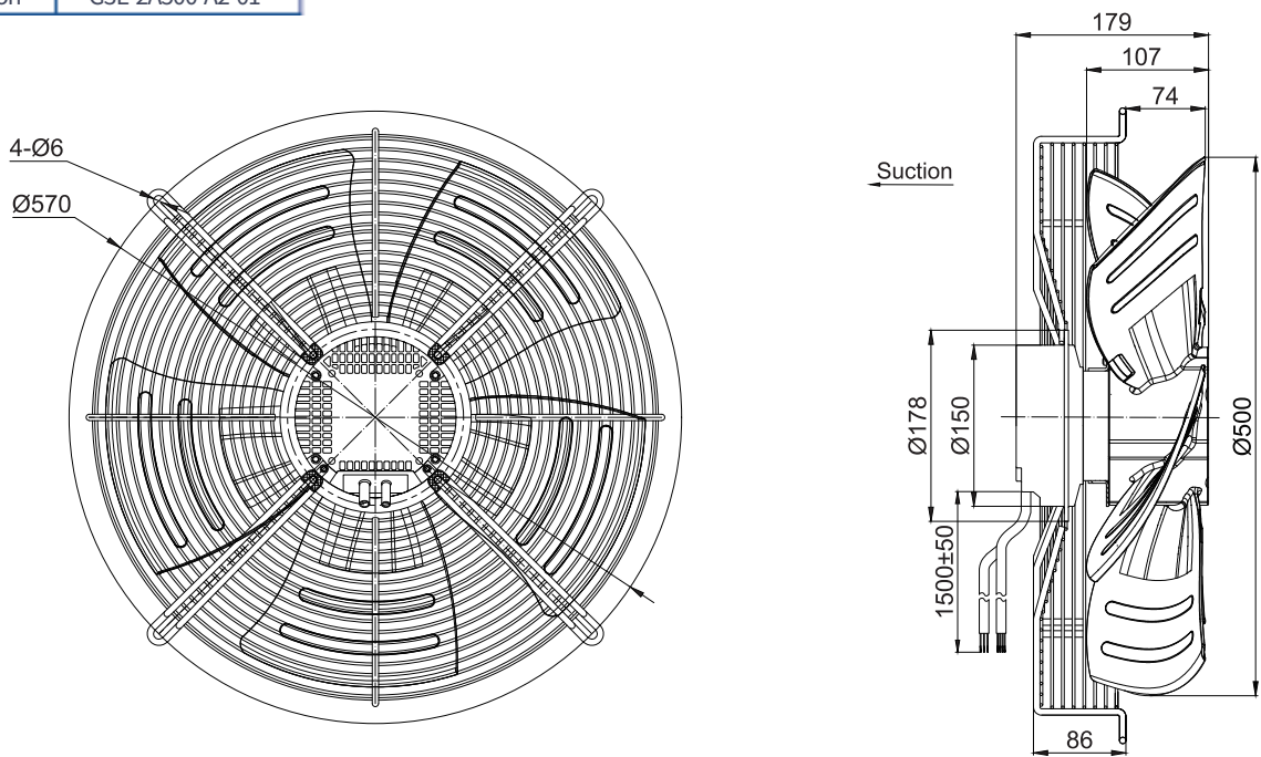
Dimensions With wall concave net cover grill
